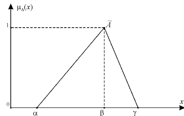
Fig. 3. Triangular membership function
