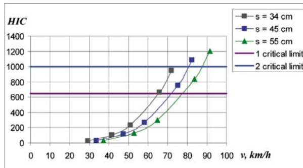
Fig. 5. HIC dependability on velocity (VW Golf)
